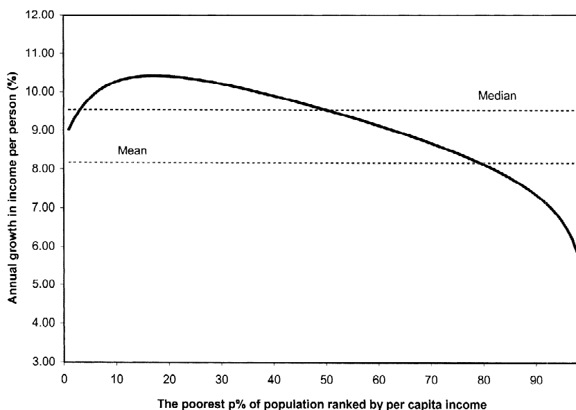
Fig. 2. Growth incidence curve for China, 1993–1996.
