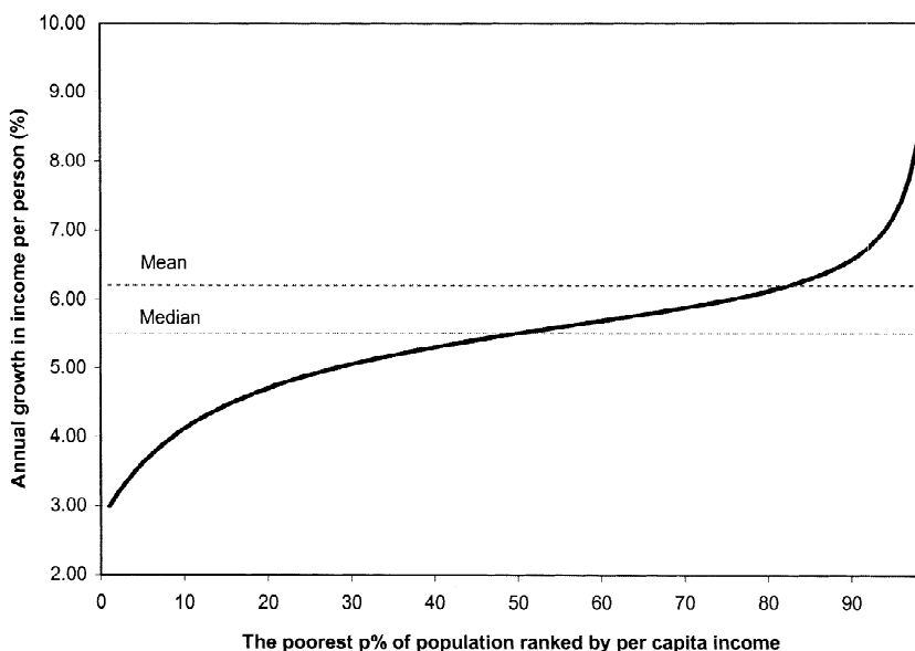
Fig. 1. Growth incidence curve for China, 1990–1999.
